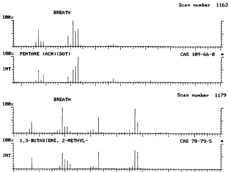
FIGURE 3 Mass spectra of chromatographic peaks. These spectra confirm the identity of pentane (upper panel) and isoprene (2-methyl-1,3-butadiene) (lower panel) in the peaks eluting at scans 1163 and 1179 respectively.
